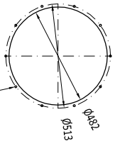
INLET FLANGE DETAIL
