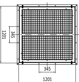
INLET FLANGE DETAIL
