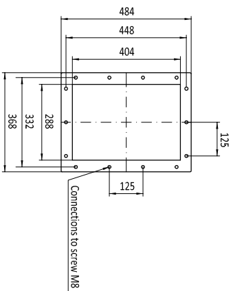
OUTLET FLANGE DETAIL
