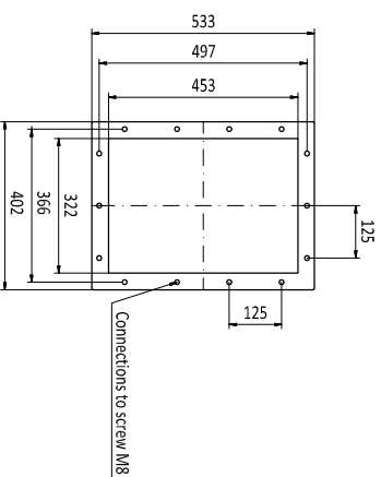
INLET FLANGE DETAIL
