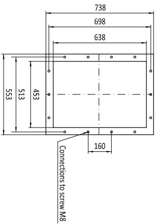
OUTLET FLANGE DETAIL
